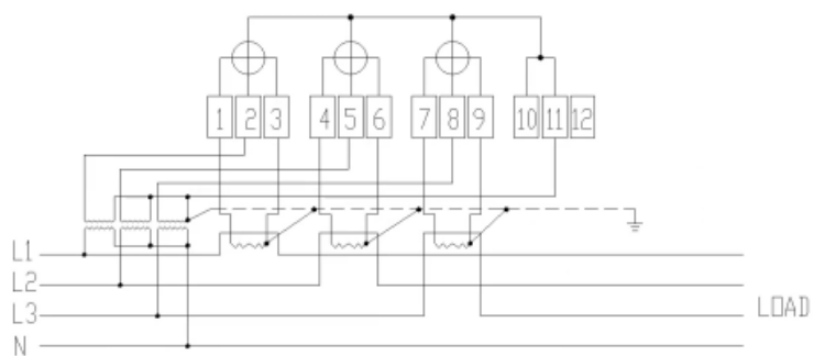
3P4W Asymmetric Connection with CT
