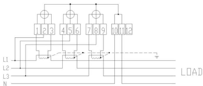
3P4W Asymmetric Connection with CT
